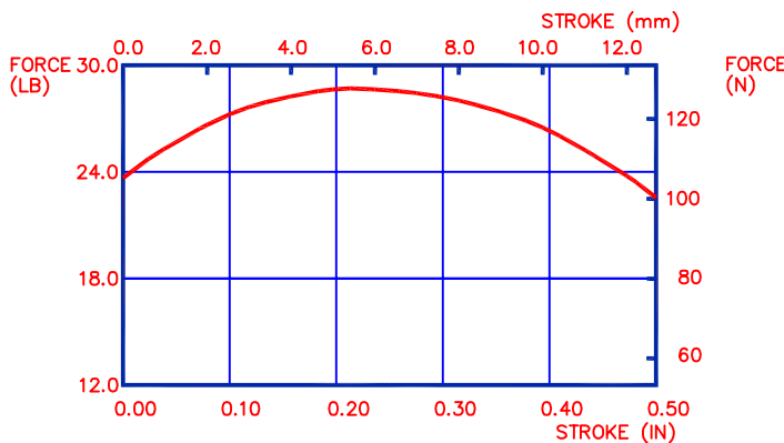
CONTINUOUS FORCE
